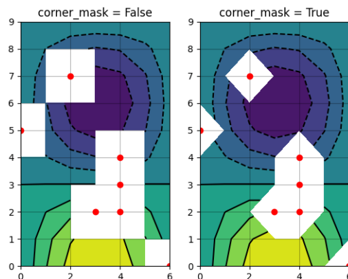
Fig. 6: Contour Corner Mask
