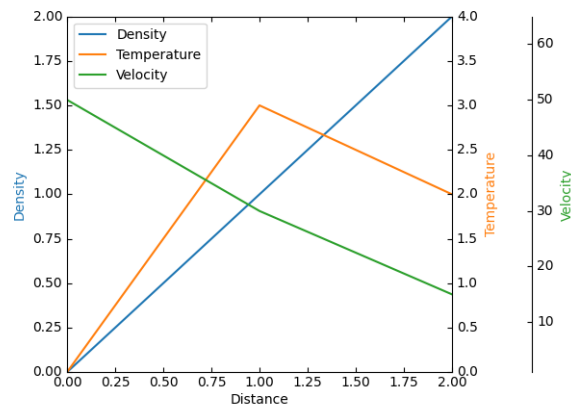
Fig. 60: Demo Parasite Axes2
